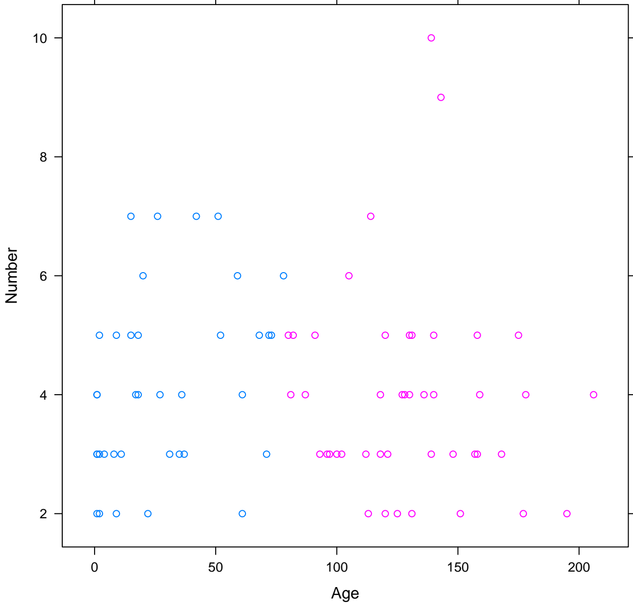
Scatterplot of kyphosis data
