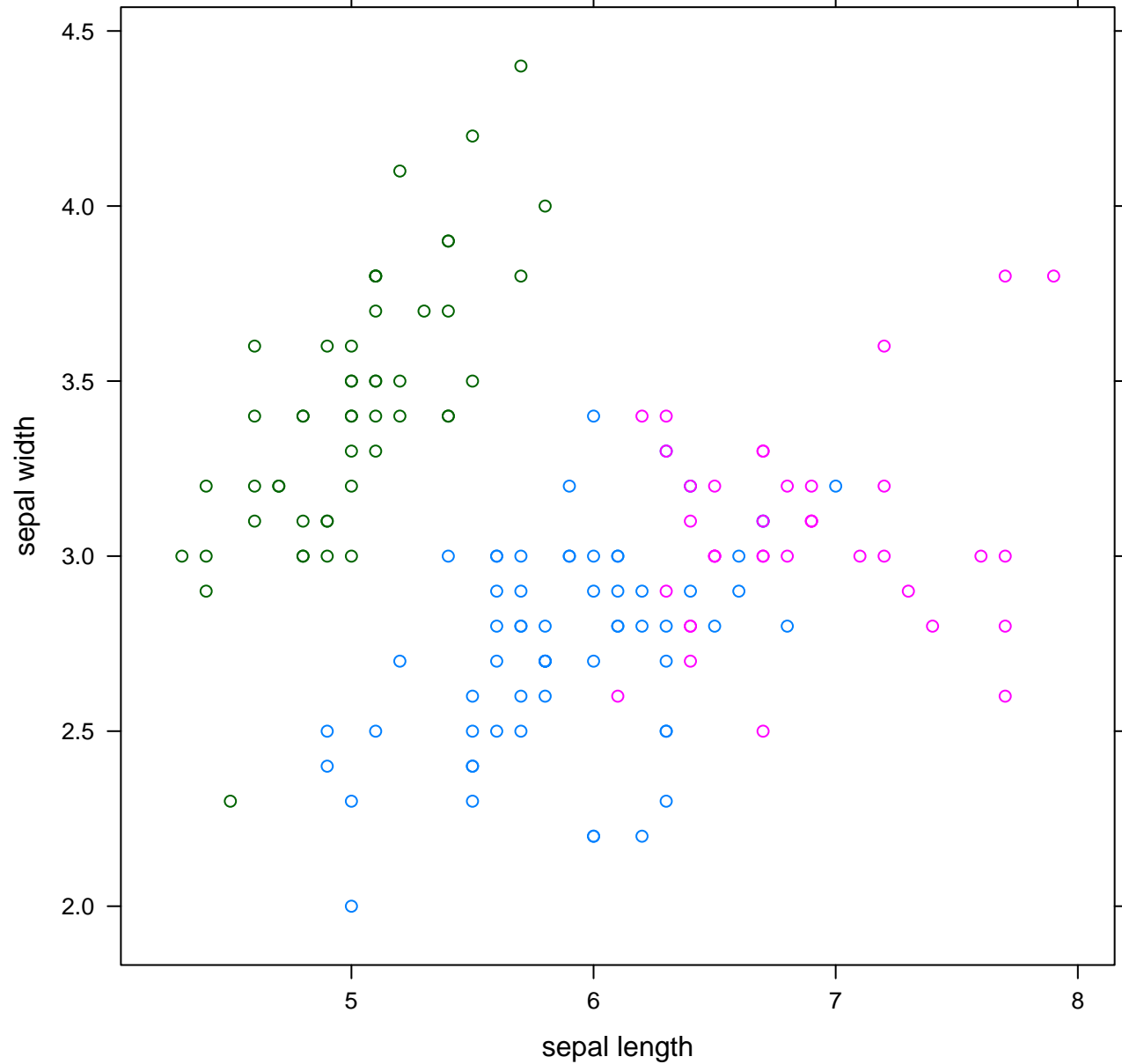
Scatterplot of iris data
